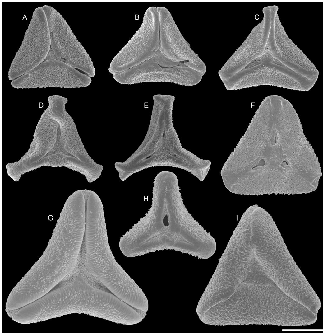
Figure 4 SEM micrographs of fossil Loranthaceae pollen with affinity to Elytrantheae and extant representatives. (A–F) Polar views of fossil pollen. (G–I) Polar views of extant pollen. (A, B) Profen MT2. (C) Profen MT3. (D, E) Profen MT4. (F). Profen MT5. (G) Peraxilla tetrapetala . (H) Amylothea sp. (I) Ligaria cuneifolia . Scale bar: (A–I) = 10 \mu\text{m} .
